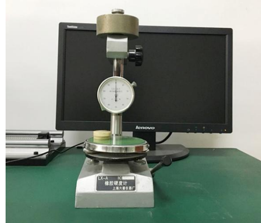
Hardness instrument
